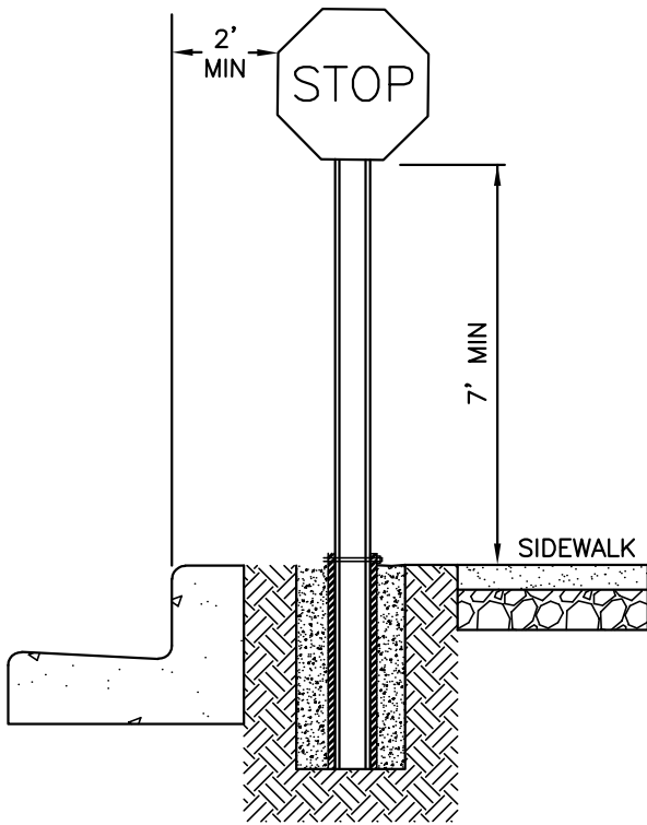
INSTALLATION BETWEEN CURB AND SIDEWALK
