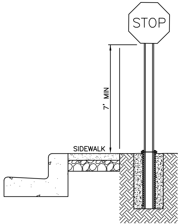
INSTALLATION BEHIND SIDEWALK
